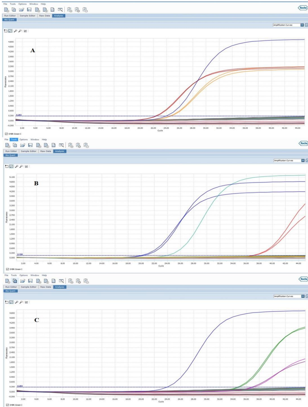
Supplementary Fig. 1. The results of SYBR Green real-time PCR tests. Each graph is depicted based on the indicated counties; A) Agh-ghala, B) Gonbad-e-Kavoos, C) Kalaleh. The technical repeats of each sample are shown with the same color.
